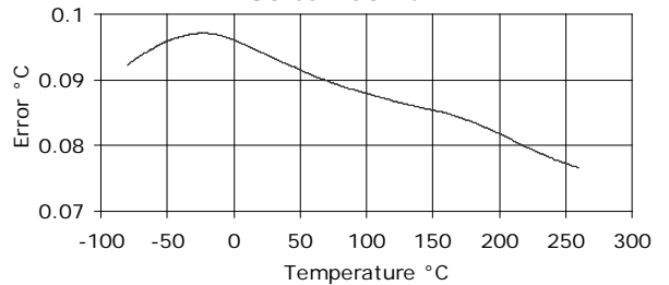
Ni120 TCR=0.00672 -80 to 260 °C
