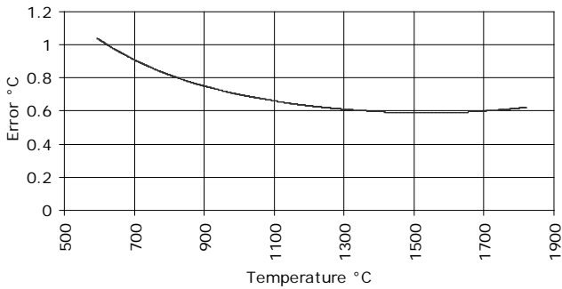
TYPE B 594 to 1820 °C
