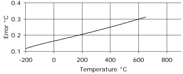
Pt100 TCR=0.003902 -200 to 648.9 °C
