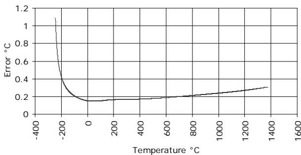
TYPE K -245 to 1372 °C
